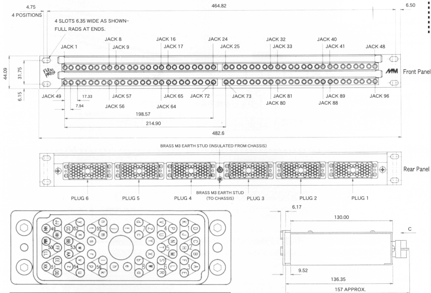
PLUG TO JACK CONNECTIONS.(MINIATURE 440 TYPE JACKS)
